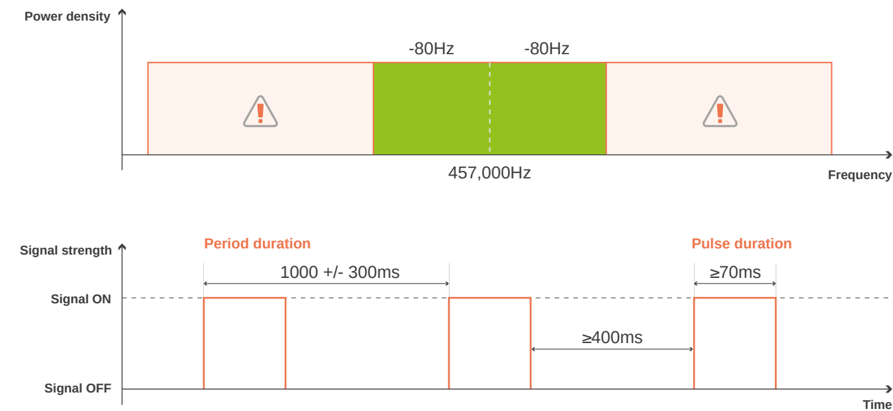
Illustration 26 Frequency deviation, Period and Pulse Duration
